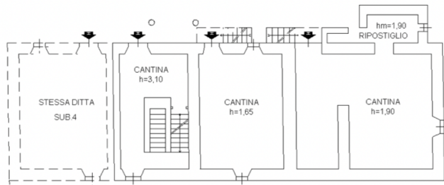
PIANO INTERRATO
